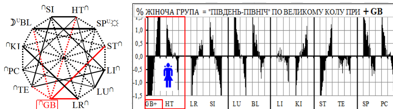
Fig.2.7 Matrix identification of systemic dependency (MIDDAY-MIDNIGHT) under +GB
