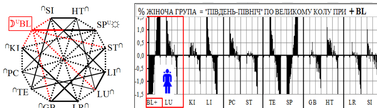
Fig.2.1 Matrix identification of systemic dependency (MIDDAY-MIDNIGHT) under +BL
