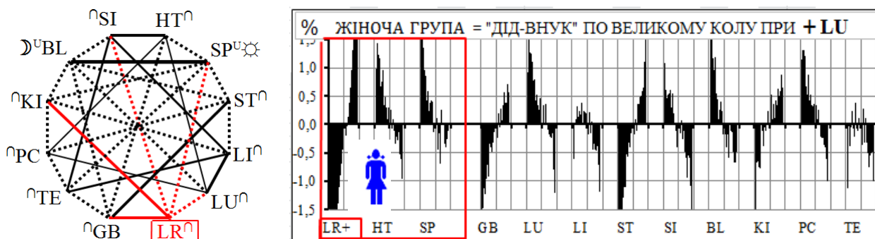
Fig.1.12 Matrix identification of systemic dependency "GRANDFATHER-GRANDSON" at +LR
