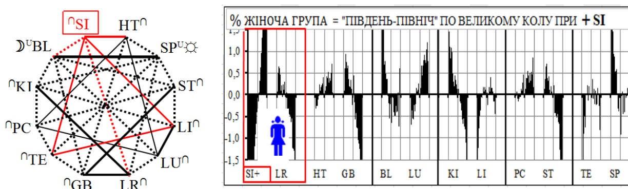
Fig.2.5 Matrix identification of systemic dependency (MIDDAY-MIDNIGHT) under +SI
