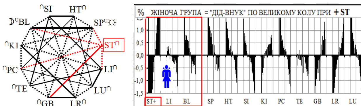
Fig.1.9 Matrix identification of systemic dependency "GRANDFATHER-GRANDSON" at +ST
